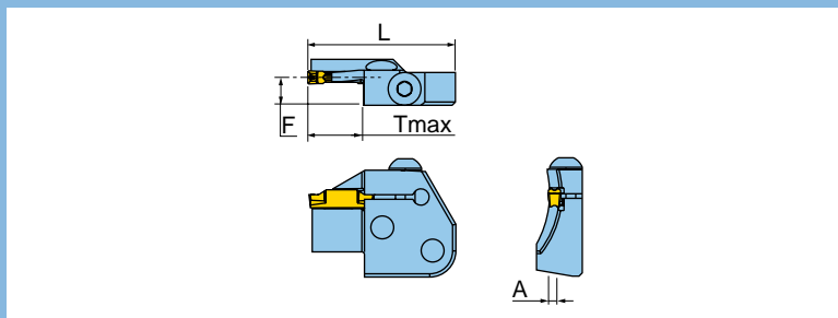
Face Turning
