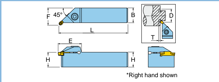
OD Undercutting
