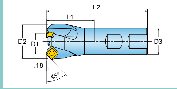
Facing
