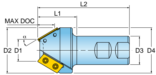
Chamfer
