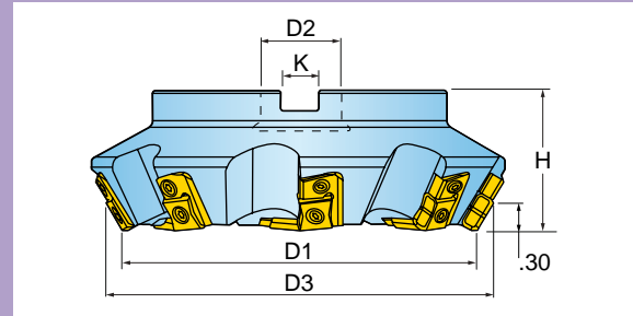
Chamfer
