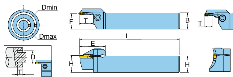
Face Turning
